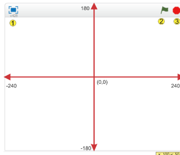
Figura 22 – Palco
