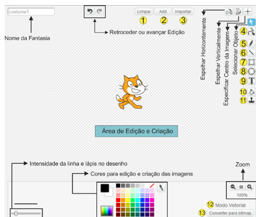
Figura 32 – Paint Editor
